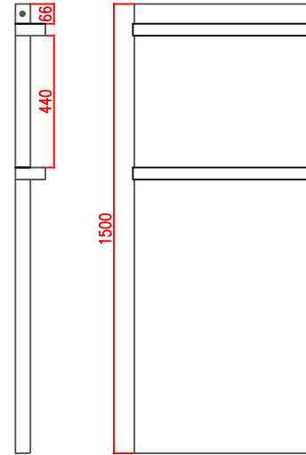
2 Rail Option
