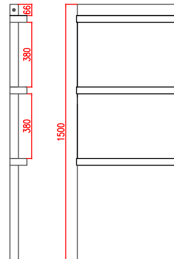
3 Rail Option
