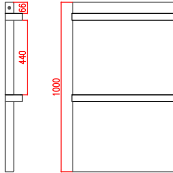
2 Rail Option
