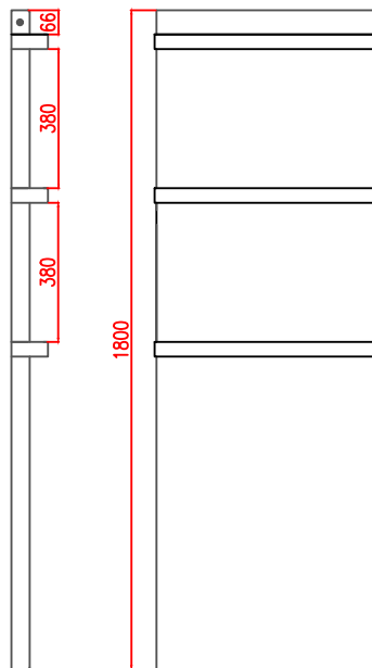
3 Rail Option
