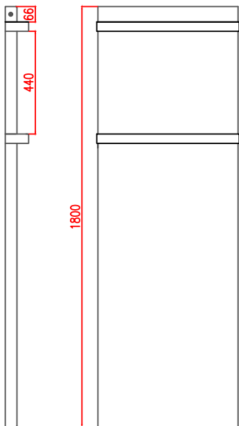
2 Rail Option
